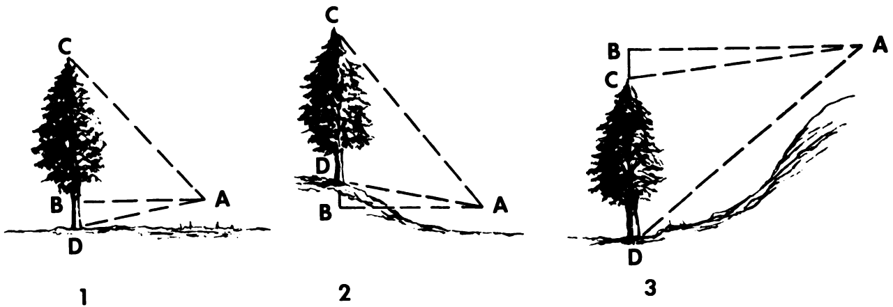
Figure 2-1. The Abney hand level.
